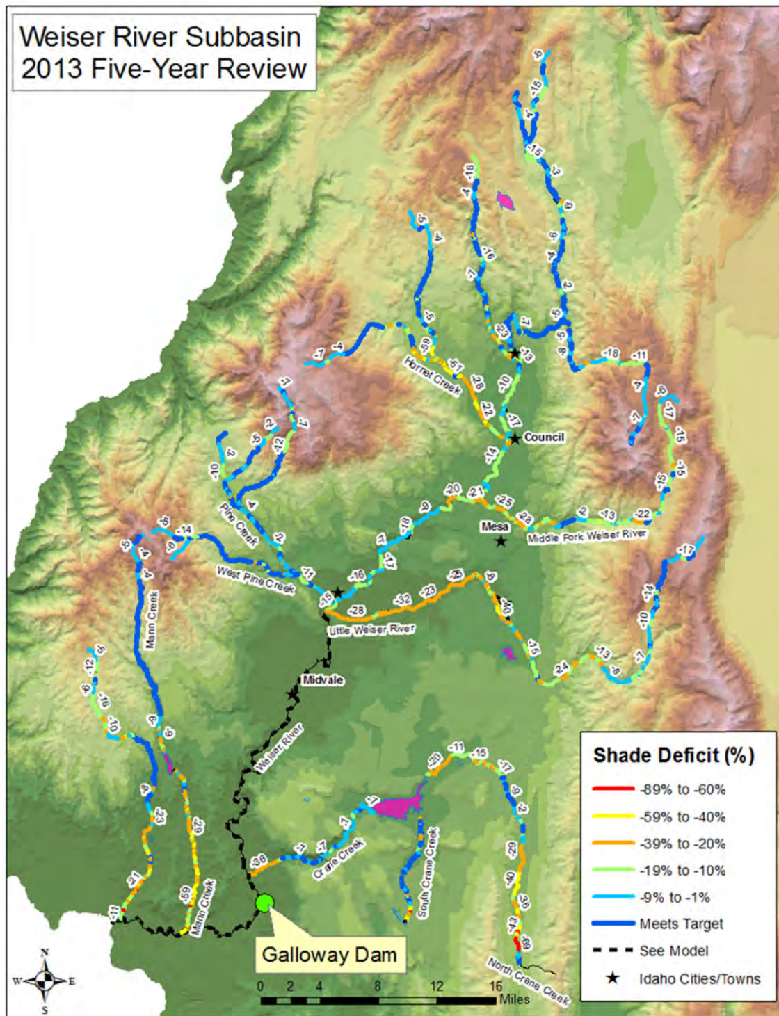
Figure 6. Shade deficits (difference between existing and target) for Weiser River subbasin in 2012.
