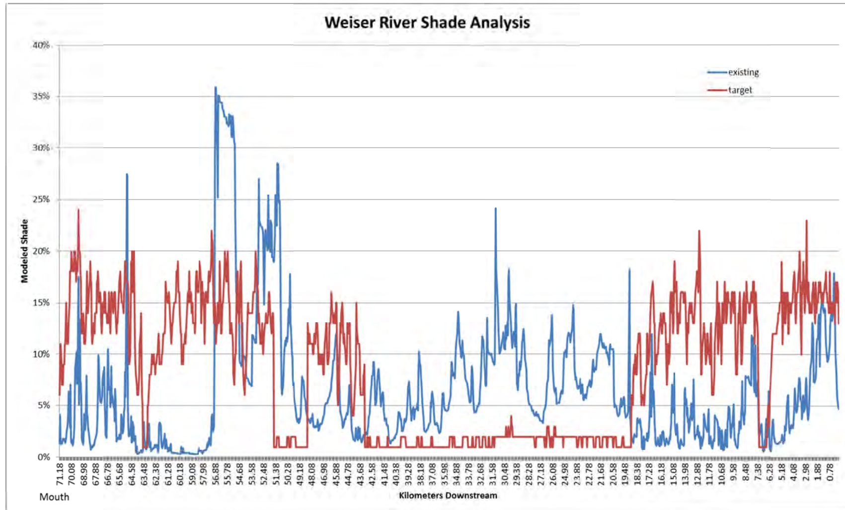
Figure 9. Existing and target shade as modeled every 50 meters for the lower Weiser River (Little Weiser River to mouth).
