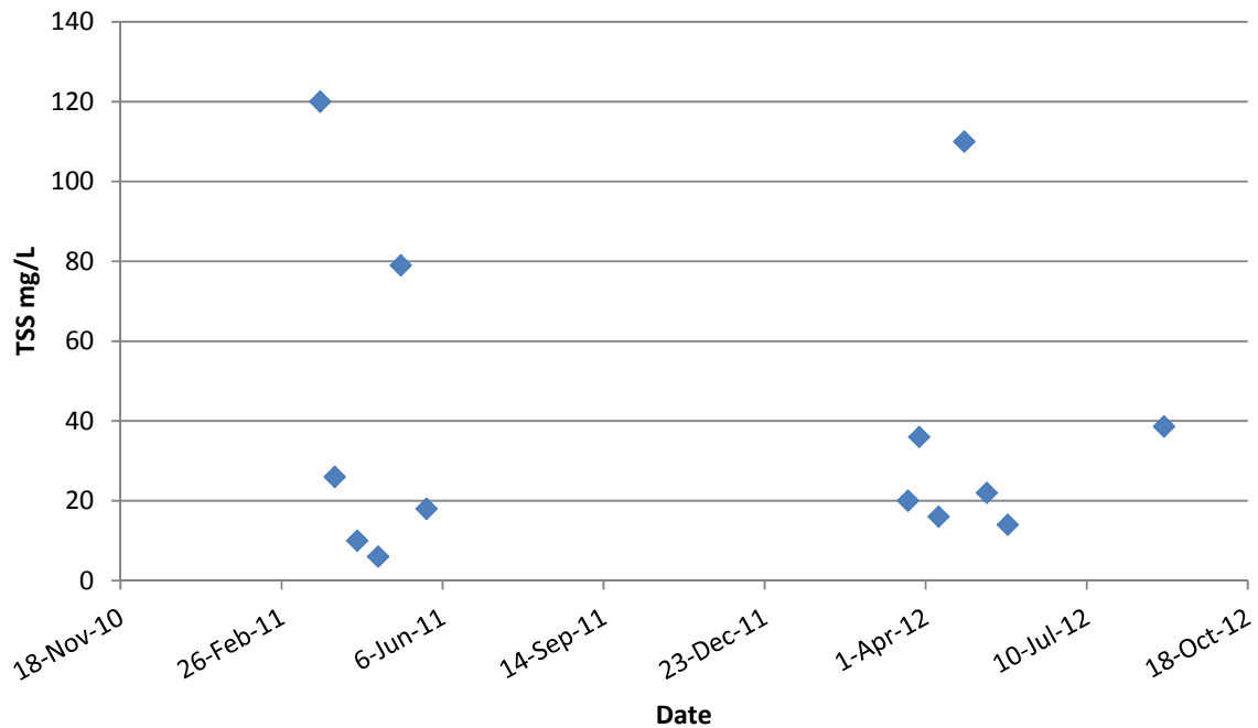
Figure 17. Total suspended solids at Galloway Dam, Weiser River for 2011–2012.
