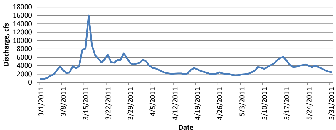
Figure 14. Discharge for the Weiser River at USGS Gage 1326600 near Weiser, Idaho, March 1, 2011 to May 31, 2011.
