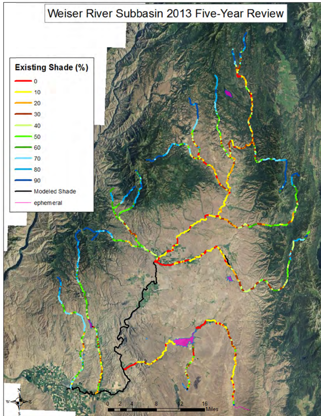
Figure 5. Existing shade estimated for Weiser River subbasin by aerial photo interpretation in 2012.
