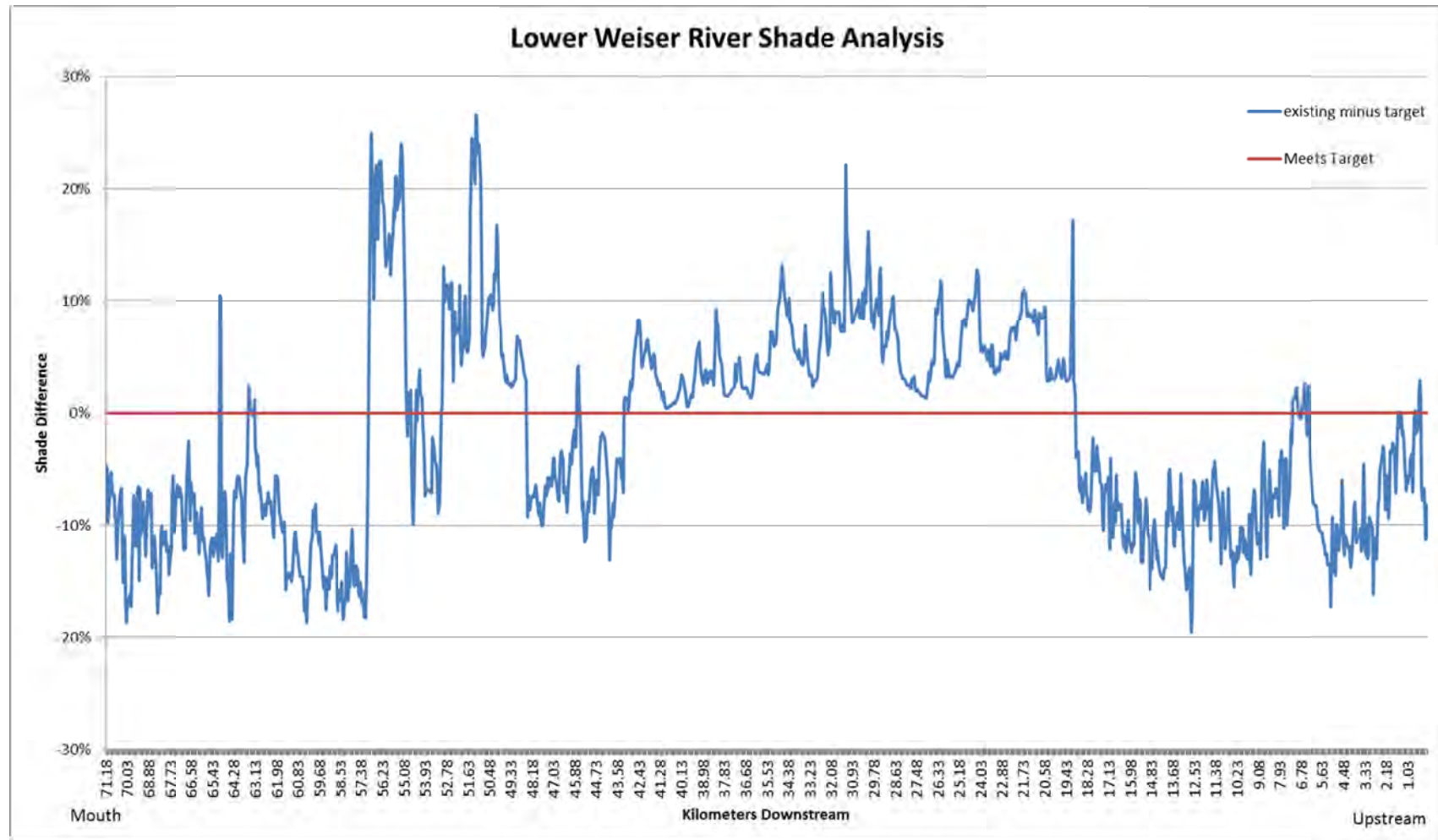
Figure 10. Shade deficit analysis as modeled every 50 meters for the lower Weiser River (Little Weiser River to mouth).
