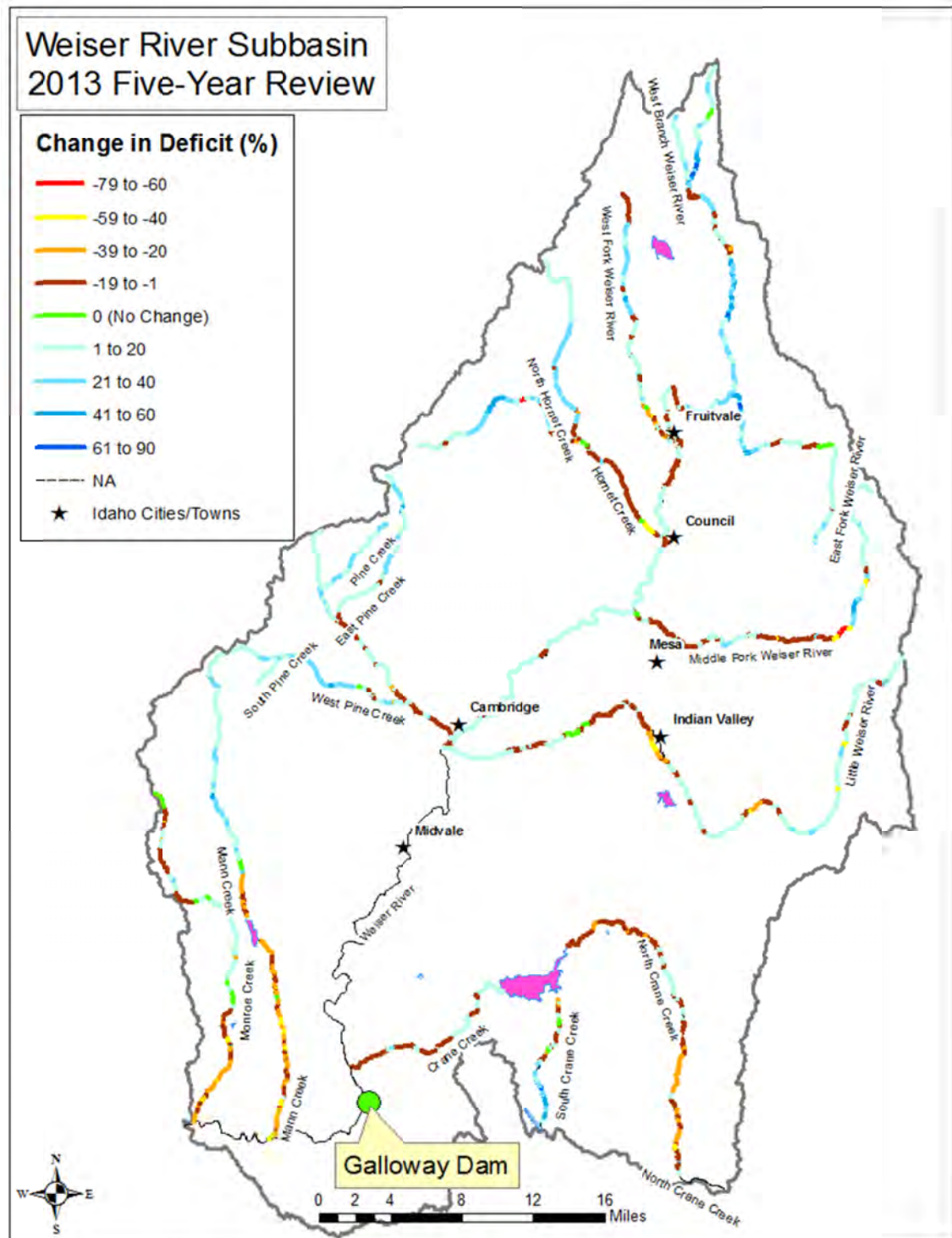
Figure 8. Changes in shade deficits from 2006 to 2012.
