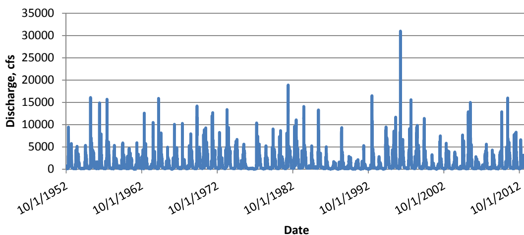
Figure 13. Historic flow (1952–present) for Weiser River at USGS Gage 1326600 near Weiser, Idaho.
