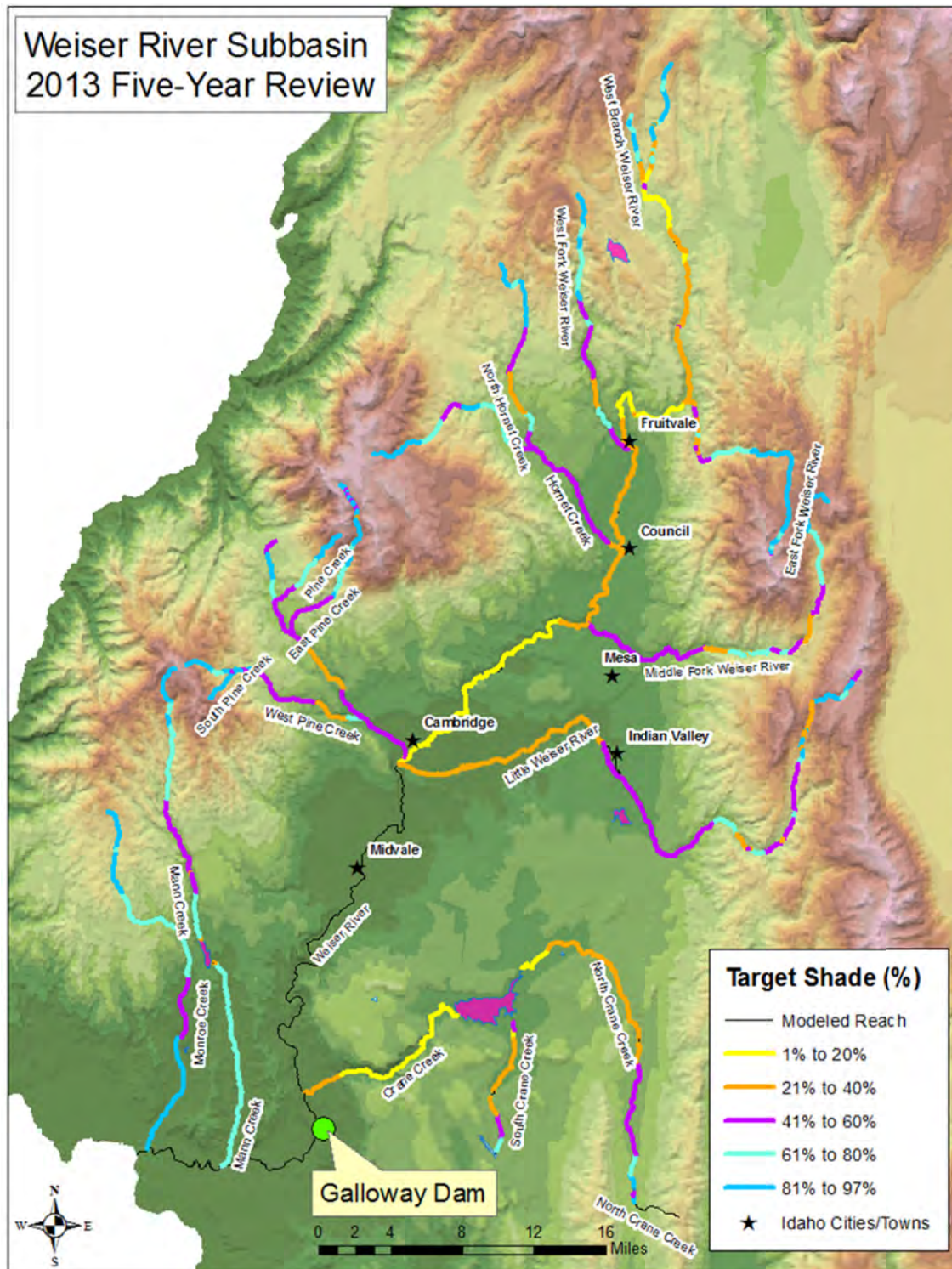
Figure 4. Target shade (2012) for Weiser River subbasin.
