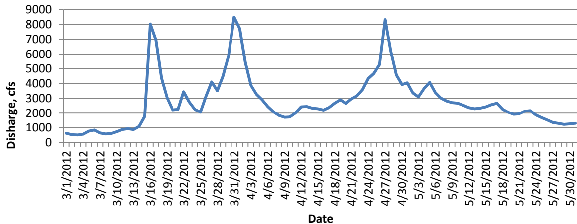
Figure 15. Discharge for the Weiser River at USGS Gage 1326600 near Weiser, Idaho, March 1, 2012 to May 31, 2012.
