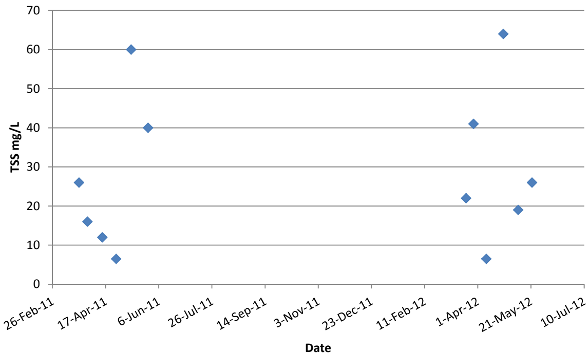
Figure 20. Total suspended solids for the Little Weiser River, 2011–2012.
