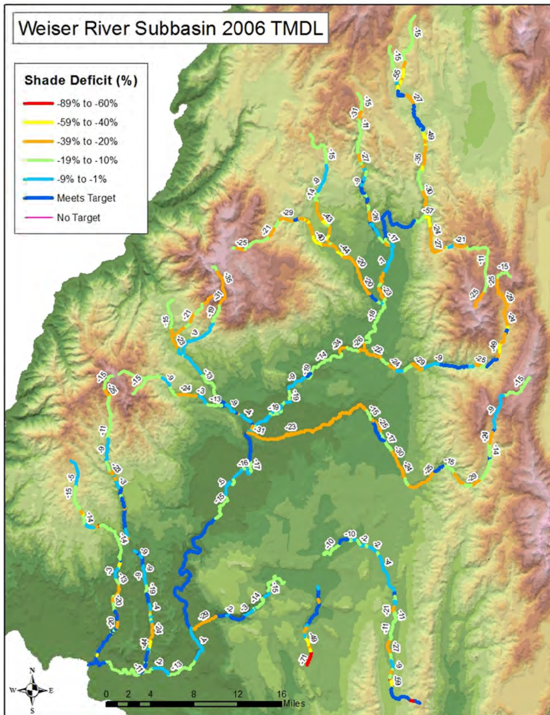
Figure 7. Shade deficits for the Weiser River subbasin in 2006 (DEQ 2006b).
