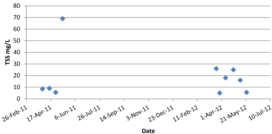
Figure 18. Total suspended solids in Crane Creek near confluence with Weiser River, 2011–2012.
