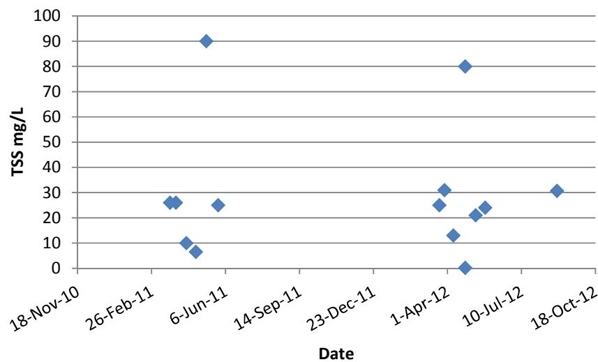
Figure 19. Total suspended solids for Weiser River at Midvale, Idaho, 2011–2012.
