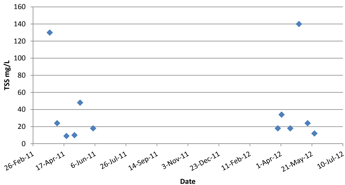
Figure 16. Total suspended solids at Weiser River at Weiser, Idaho, 2011–2012.
