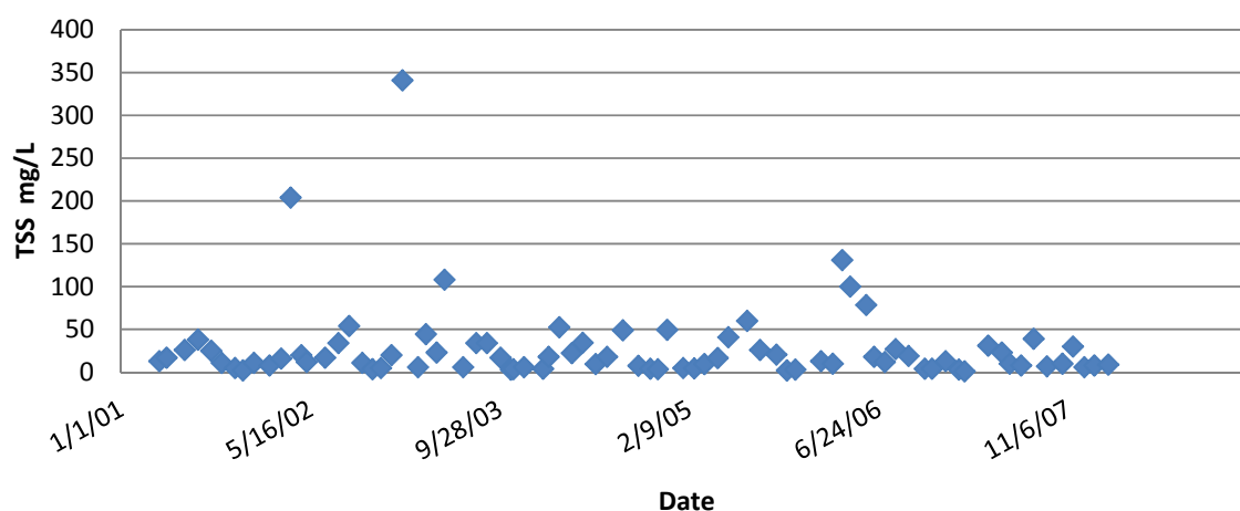
Figure 21. Bureau of Reclamation total suspended solids data on the Weiser River at Weiser, Idaho, 2001–2008.
