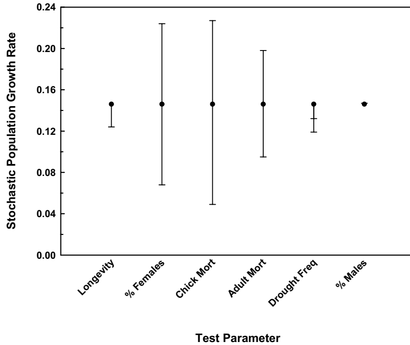
Fig. 31. Demographic sensitivity analysis of a simulated GUSG population. Stochastic population growth rate for a set of models in which the specific parameter is varied across a range of biologically plausible values. The baseline model growth rate of 0.146 is given by the central data point for each parameter. The general model of sage-grouse population dynamics is most sensitive to uncertainty in those parameters giving the widest range in simulated population growth rates.
