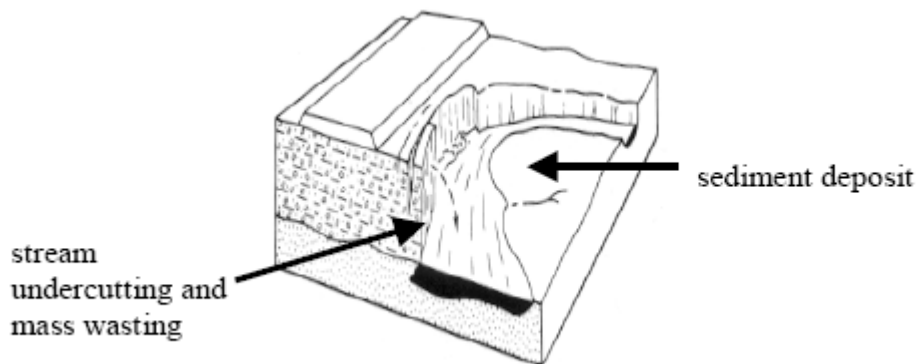
Figure 12. Outer edge of a meander bend showing mass wasting on the outside of the bend and deposition on the inside (adapted from Varnes, 1978).
